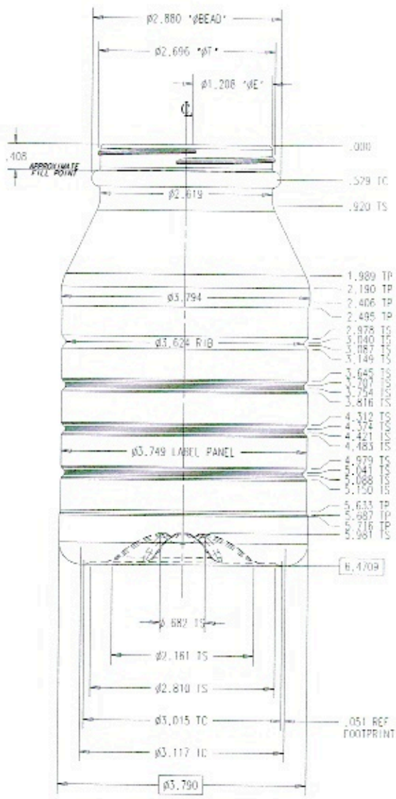
FRONT VIEW
