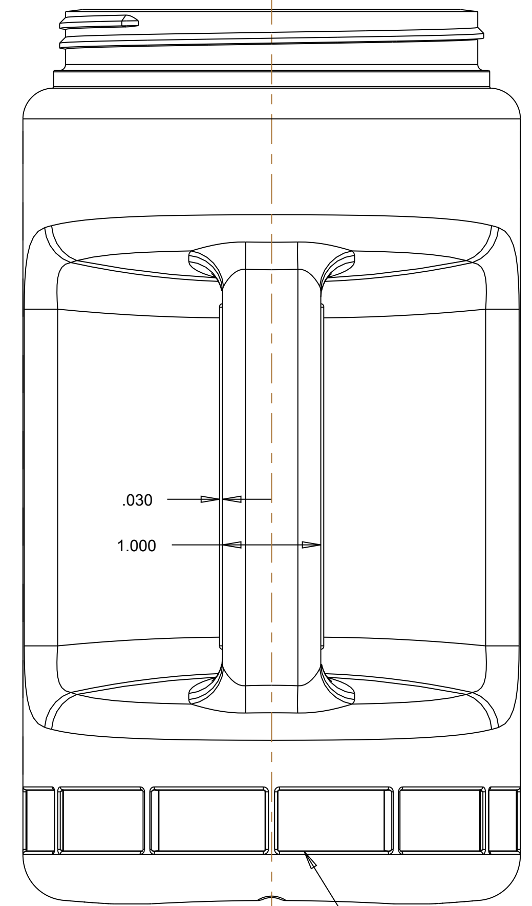
(12) RECTANGULAR PATTERN .040 DEEP EQUALLY SPACED
