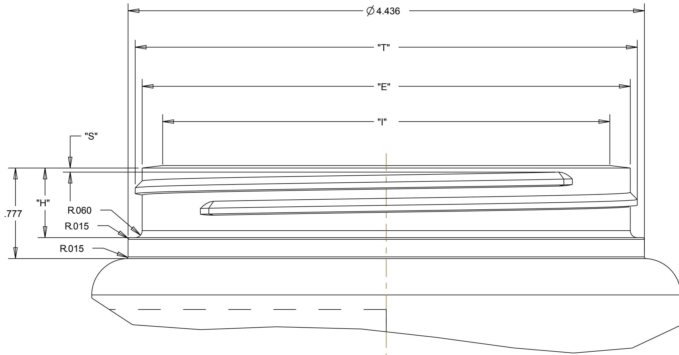
DETAIL A SCALE 2.000
